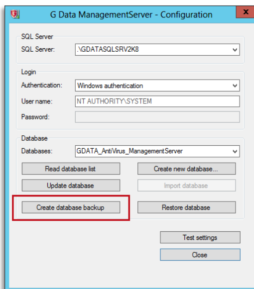
Figure 1: GdmsConfig.exe
